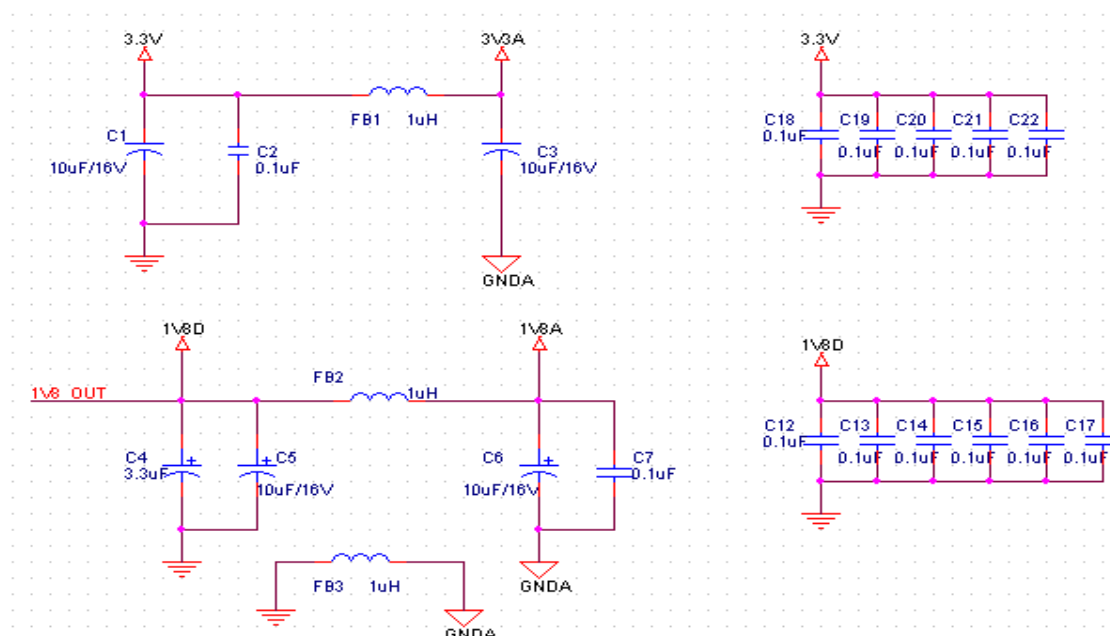
Fig 2. Power Design
