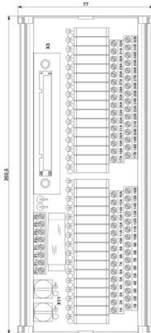
Dimensional drawing
