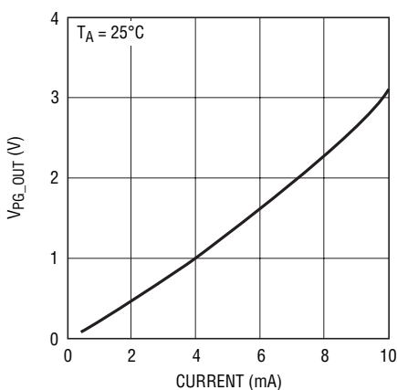
Power Good Output Low Voltage vs Current
