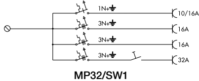
Wiring diagram
