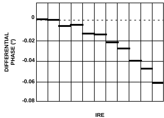
FIGURE 16. DIFFERENTIAL PHASE
