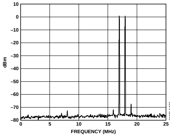
Figure 27. Dual-Tone Spectral Plot of TxDAC's Output ( f_{\text{DATA}} = 50 \text{ MSPS} , 4× Interpolation, 10 dBm Peak Power, F1 = 17 \text{ MHz} , F2 = 18 \text{ MHz} )
