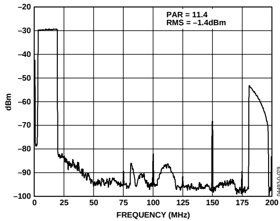
Figure 34. Wideband Spectral Plot of 88-Subcarrier OFDM Test Vector ( f_{\text{DATA}} = 50 \text{ MSPS} , 4× Interpolation)
