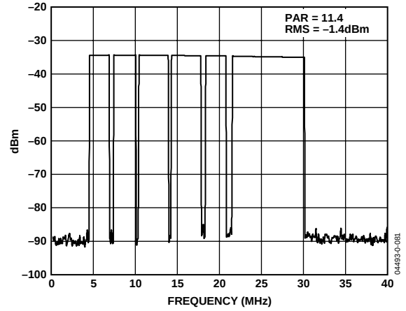
Figure 36. Spectral Plot of 111-Carrier OFDM Test Vector ( f_{\text{DATA}} = 80 \text{ MSPS} , 2× Interpolation)
