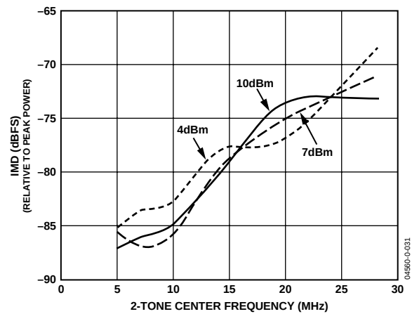
Figure 31. 2-Tone IMD Frequency Sweep vs. Peak Power with f_{\text{DATA}} = 80 \text{ MSPS} , 2× Interpolation
