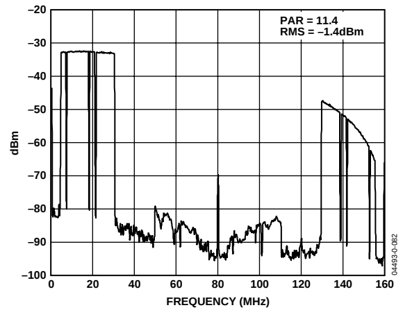
Figure 37. Wideband Spectral Plot of 111-Carrier OFDM Test Vector ( f_{\text{DATA}} = 80 \text{ MSPS} , 2× Interpolation)
