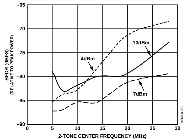
Figure 32. 2-Tone Worst Spur Frequency Sweep vs. Peak Power with f_{\text{DATA}} = 80 \text{ MSPS} , 2× Interpolation
