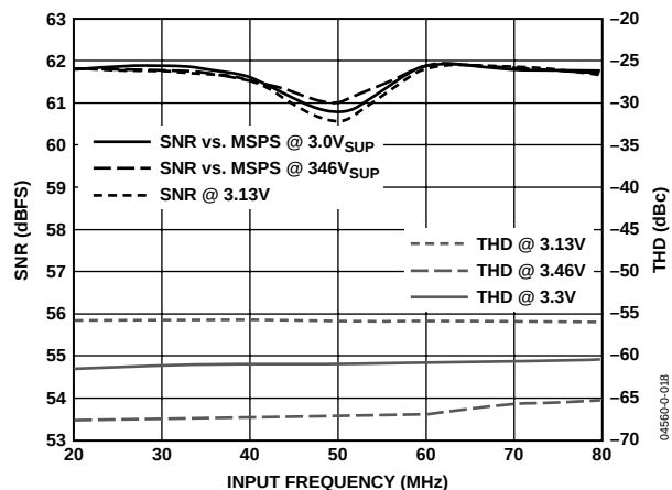
Figure 18. SNR and THD vs. Sample Rate and Supply (LPF Disabled; RxPGA = 0 dB; f_{\text{IN}} = 8 MHz)
