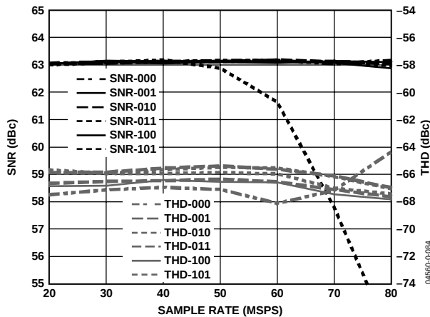
Figure 84. SNR and THD Performance vs. f_{ADC} and SPGA Bias Setting with RxPGA = 0 dB, f_{IN} = 10 MHz, A_{IN} = -1 dBFS
