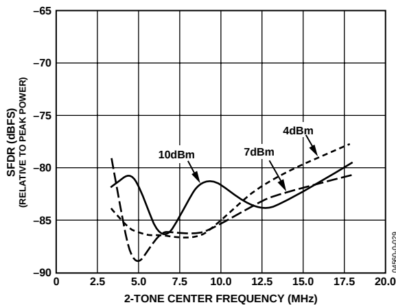
Figure 29. 2-Tone Worst Spur Frequency Sweep vs. Peak Power with f_{\text{DATA}} = 50 \text{ MSPS} , 4× Interpolation
