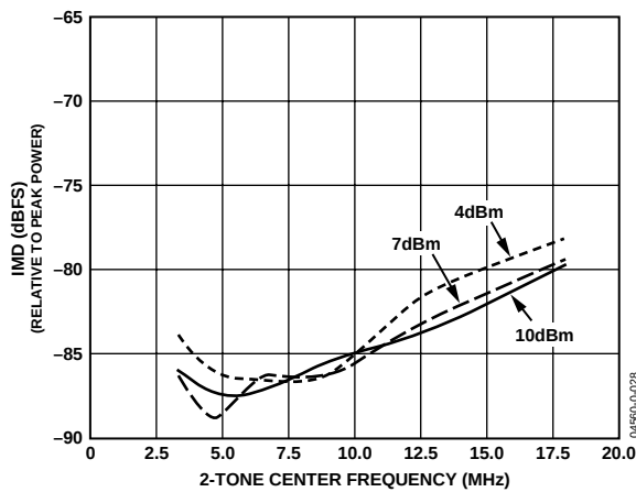
Figure 28. 2-Tone IMD Frequency Sweep vs. Peak Power with f_{\text{DATA}} = 50 \text{ MSPS} , 4× Interpolation
