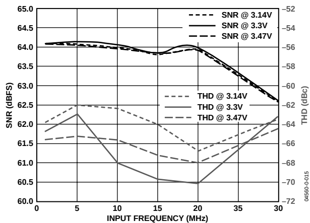
Figure 15. SNR and THD vs. Input Frequency and Supply (LPF f_{-3\text{ dB}} = 26 MHz; RxPGA = 0 dB)
