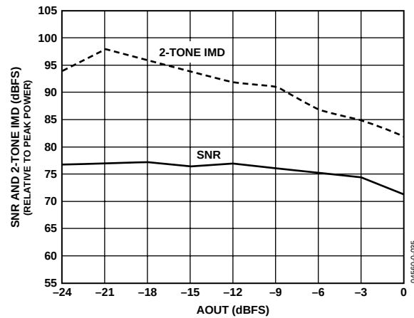
Figure 35. SNR and SFDR vs. P_{\text{OUT}} ( f_{\text{OUT}} = 12.55 \text{ MHz} , f_{\text{DATA}} = 50 \text{ MSPS} , 4× Interpolation)
