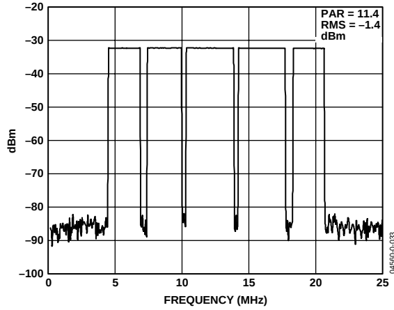
Figure 33. Spectral Plot of 84-Carrier OFDM Test Vector ( f_{\text{DATA}} = 50 \text{ MSPS} , 4× Interpolation)
