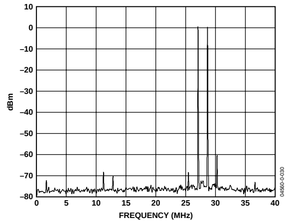
Figure 30. Dual-Tone Spectral Plot of TxDAC's Output ( f_{\text{DATA}} = 80 \text{ MSPS} , 2× Interpolation, 10 dBm Peak Power, F1 = 27.1 \text{ MHz} , F2 = 28.7 \text{ MHz} )
