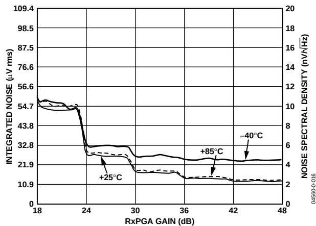
Figure 16. Input Referred Integrated Noise and Noise Spectral Density vs. RxPGA Gain (LPF f_{-3\text{ dB}} = 26 MHz)
