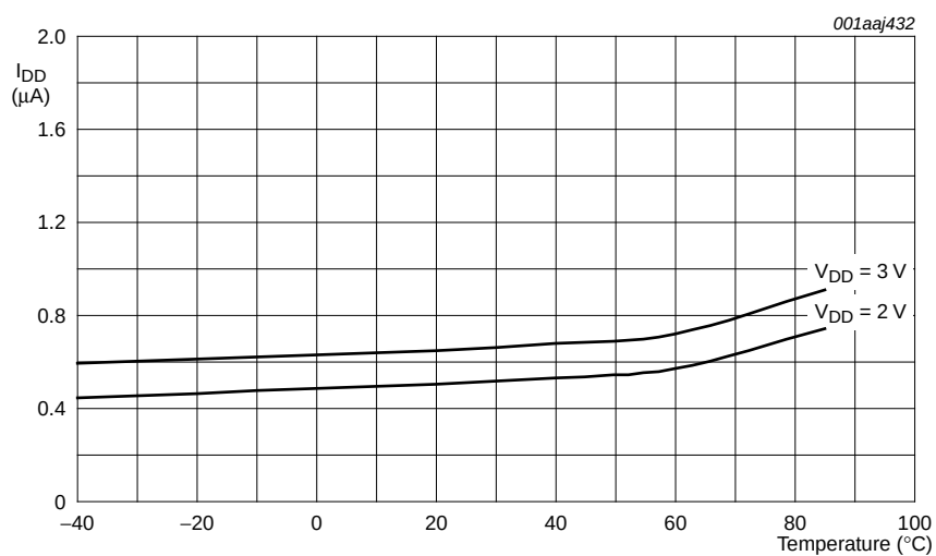
Fig 39. I DD as a function of temperature
