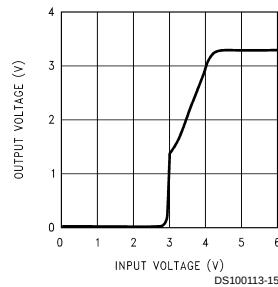
Low Voltage Behavior (3.3)
