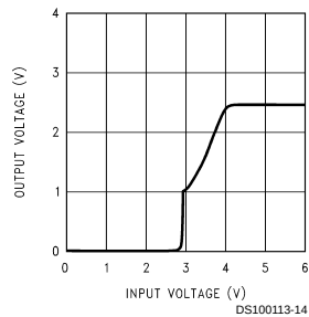
Low Voltage Behavior (2.5V)
