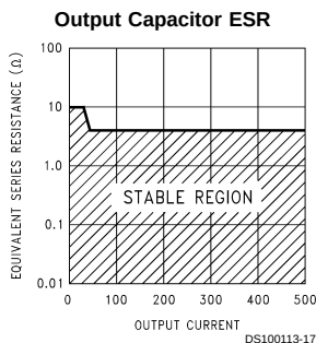
FIGURE 1. ESR Limits
