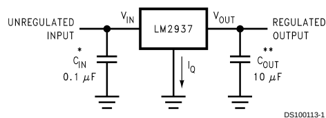
Typical Application
