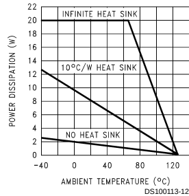
Maximum Power Dissipation (TO-220)
