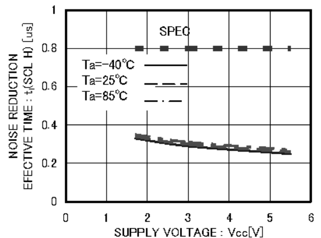
Figure 25. Noise reduction affection time tI(SCL H)
