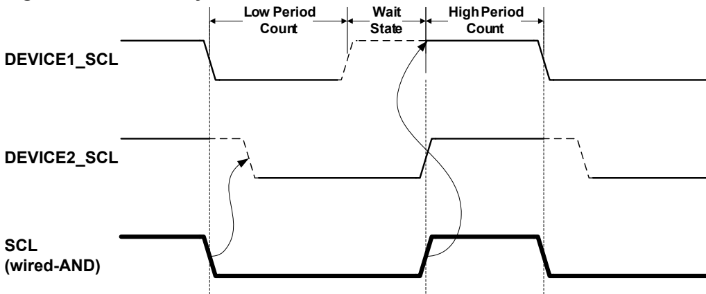
Figure 25-11. Clock Synchronization
