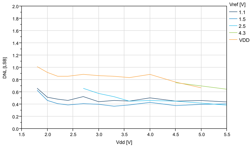
Figure 32-42. DNL Error vs. V_{DD} ( f_{ADC}=115 ksp/s) at T=25^{\circ}C , REFSEL = Internal Reference
