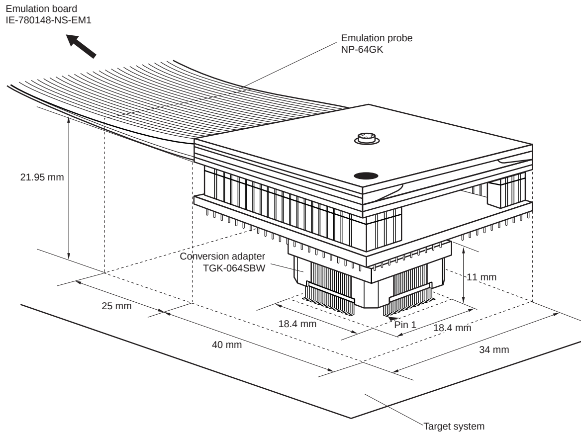
Figure B-6. Connection Conditions of Target System (When Using NP-64GK)
