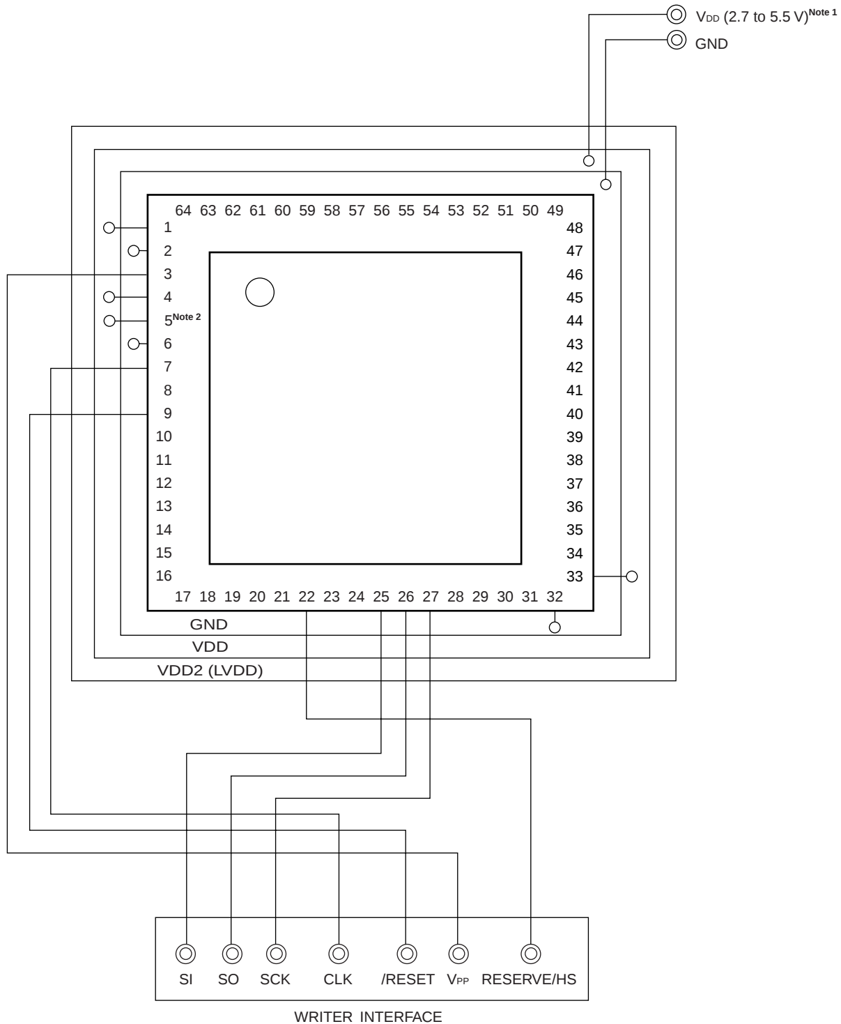
Figure 27-4. Example of Wiring Adapter for Flash Memory Writing in 3-Wire Serial I/O (CS10 + HS) Mode
