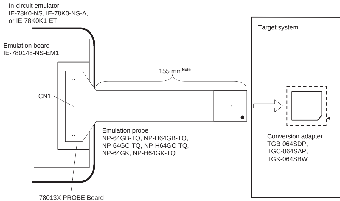
Figure B-1. Distance Between In-Circuit Emulator and Conversion Adapter
