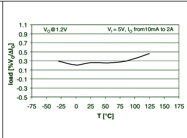
Figure 10. Load regulation vs. temperature
