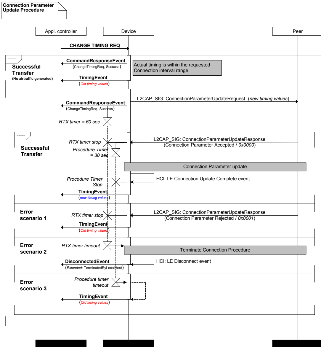
Figure 53. ChangeTimingRequest MSC
