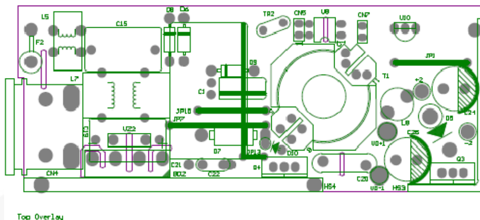
Figure 25. Top Overlay
