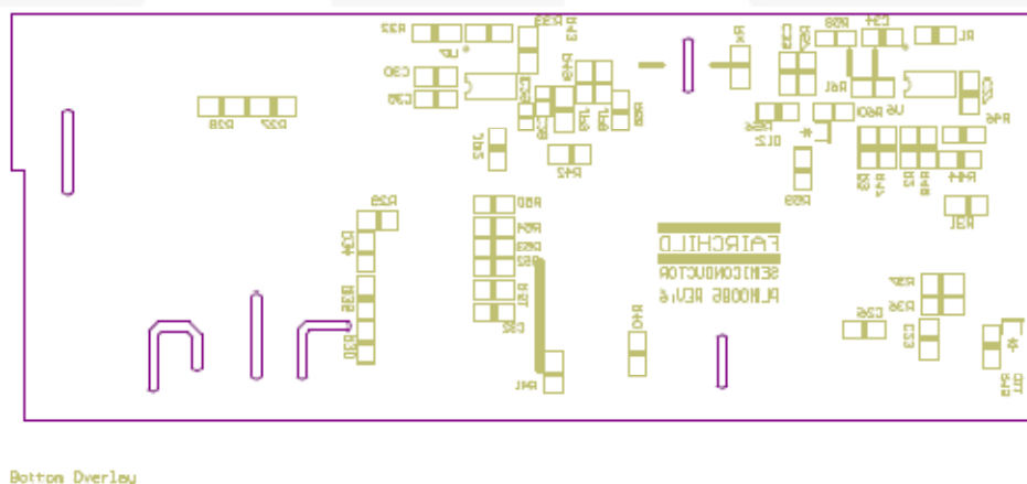
Figure 26. Bottom Overlay
