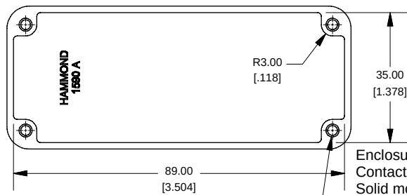
Top View Looking Inside Box
