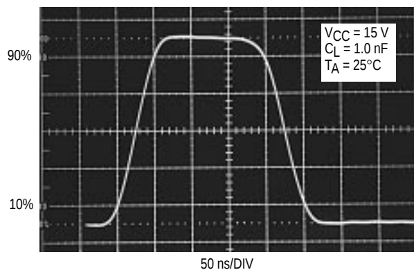
Figure 12. Output Waveform
