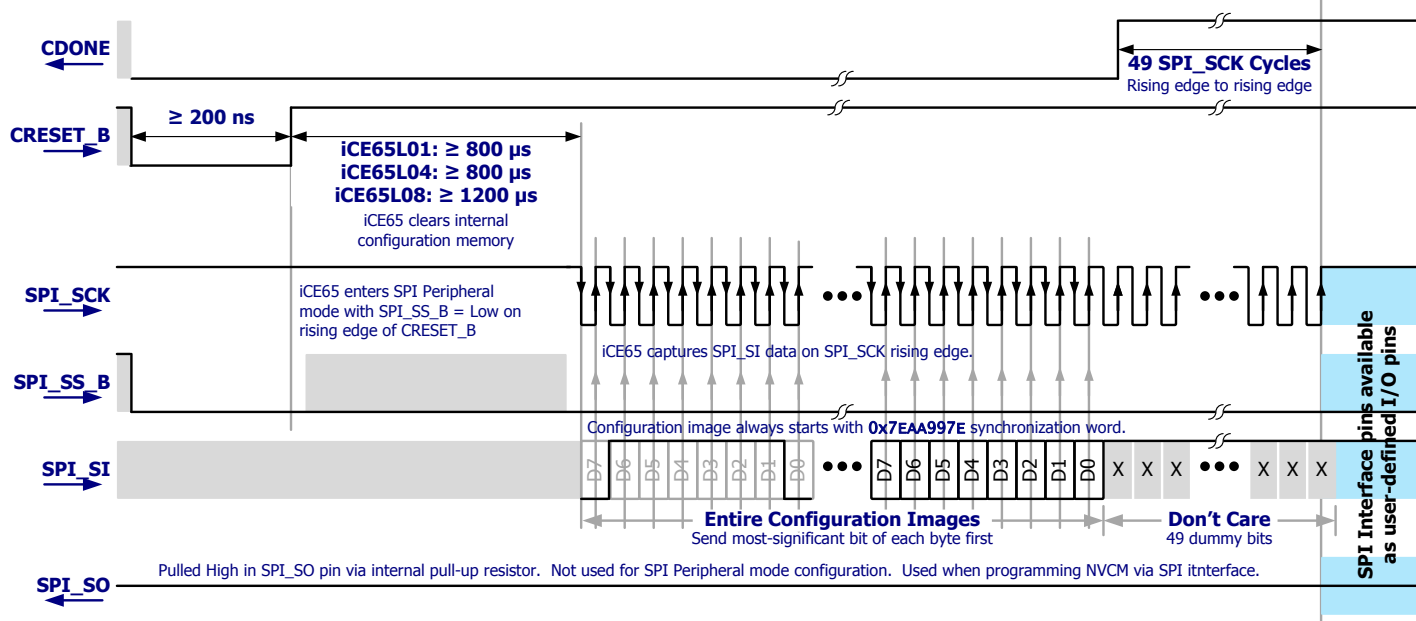
Figure 29: Application Processor Waveforms for SPI Peripheral Mode Configuration Process
