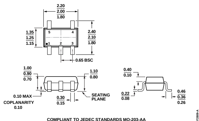
Figure 7. 5-Lead Thin Shrink Small Outline Transistor Package [SC70] (KS-5) Dimensions shown in millimeters
