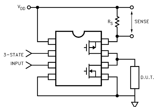
FIGURE 9. PIN DRIVER
