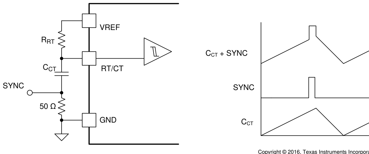
Figure 24. Oscillator Synchronization Circuit
