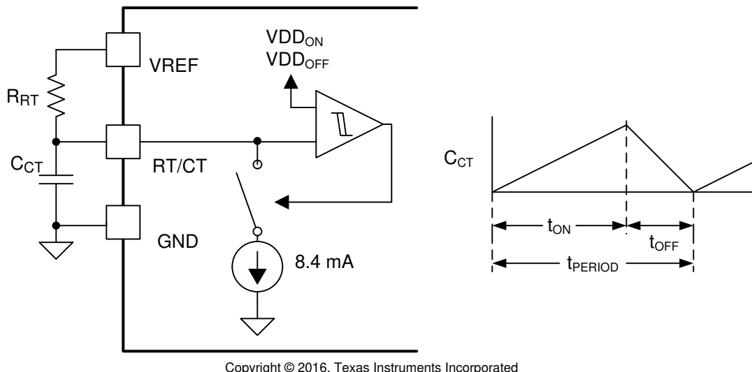
Figure 23. Oscillator Circuit
