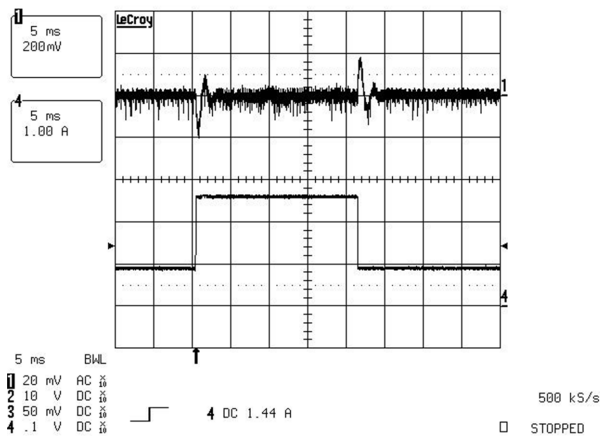
Figure 37. Output Voltage During 0.9-A to 2.7-A Load Transient
