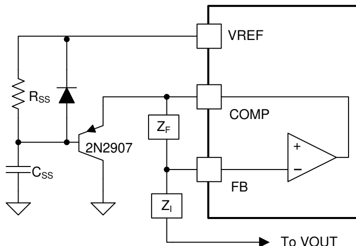
Figure 25. Soft-Start Implementation
