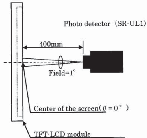
Fig. 6 The way of measuring Contrast/ Luminance/ Chromaticity
