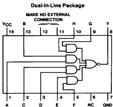
DM5454 (J) DM7454 (N)
