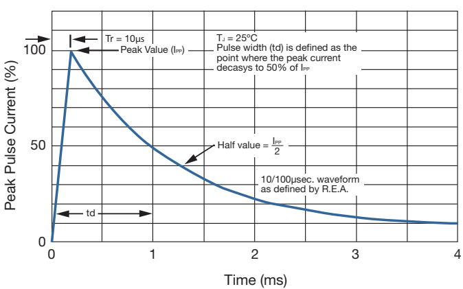
FIG 5. PULSE WAVEFORM
