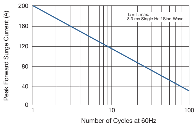
FIG 2. MAXIMUM NON-REPETITIVE
