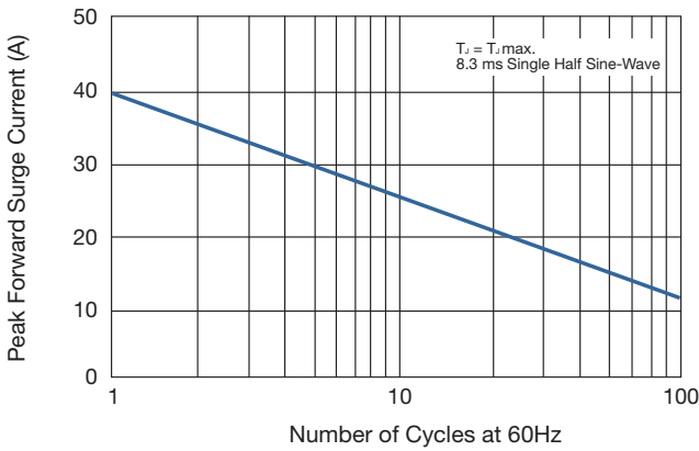
FIG 2. MAXIMUM NON-REPETITIVE
