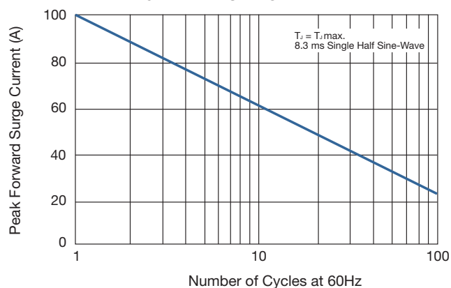
FIG 2. MAXIMUM NON-REPETITIVE
