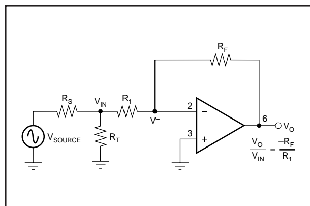
FIGURE 4. Inverting Op Amp.
