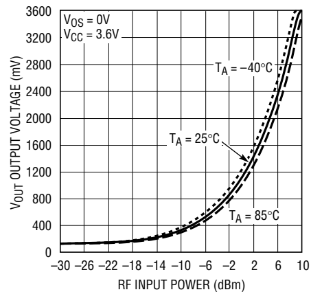
Typical Detector Characteristics, 6000MHz
