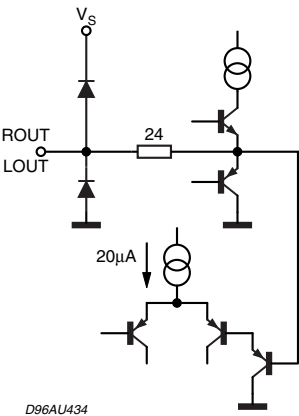
Figure 20. Pins 6, 7, 8, 9
