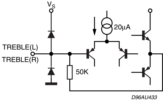
Figure 24. Pin 19
