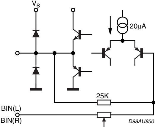
Figure 21. Pins 13, 14
