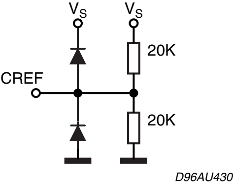
Figure 18. Pins 4, 5
