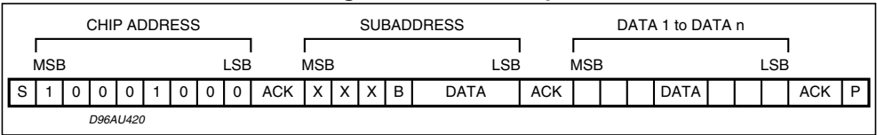
Figure 13. Interface protocol
