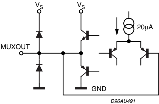
Figure 19. Pins 12, 15
