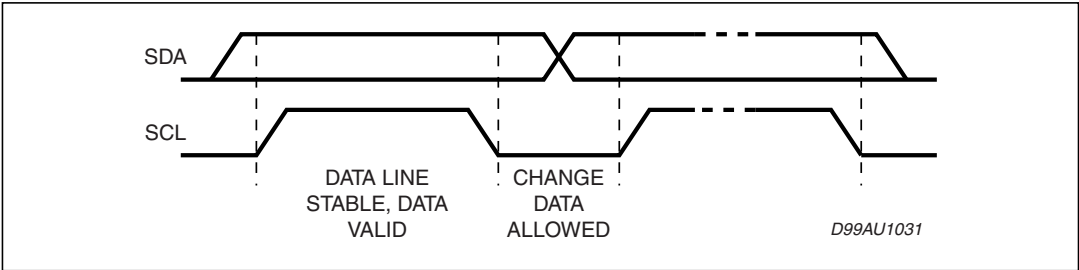
Figure 10. Data validity on the I 2 C bus
