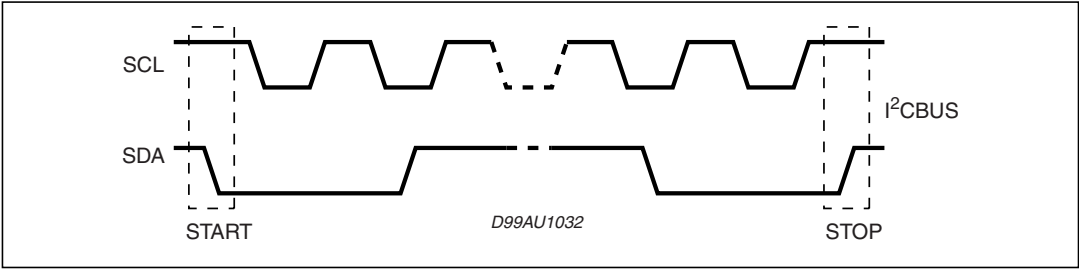
Figure 11. Timing diagram of I 2 C bus
