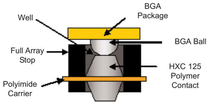
Contact to Solder Ball Interface
