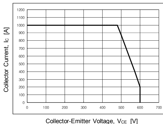
Fig 11. SCSOA Characteristic
