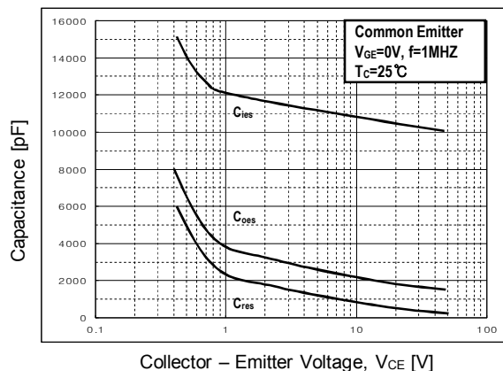
Fig 7. Capacitance characteristics
