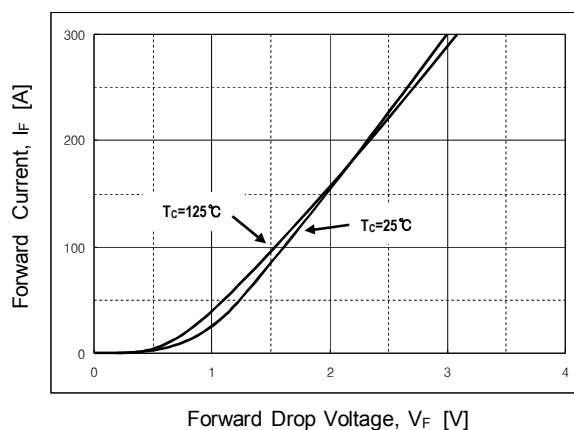
Fig 15. Forward characteristics
