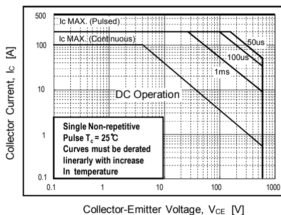
Fig14. SOA characteristics
