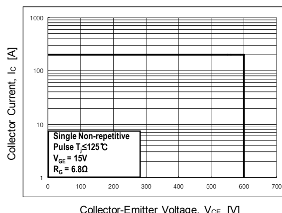
Fig 10. RBSOA Characteristic
