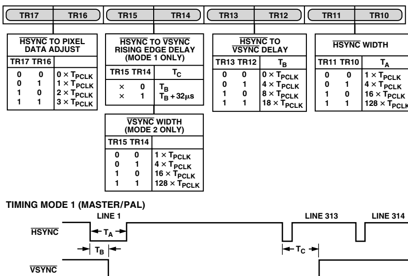
Figure 51. Timing Register 1
