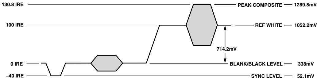
Figure 95. NTSC Composite Video Levels
