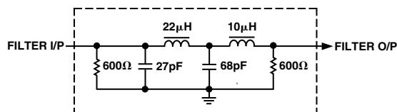
Figure 86. Output Filter for 4× Oversampling Mode
