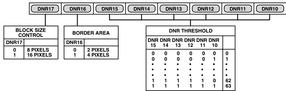
Figure 70. DNR Register 1
