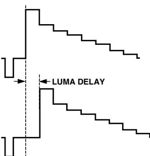
Figure 12. Luma Delay
