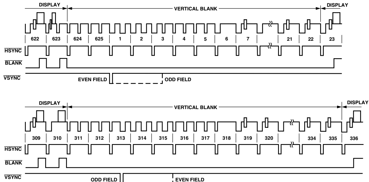
Figure 30. Timing Mode 2, PAL
