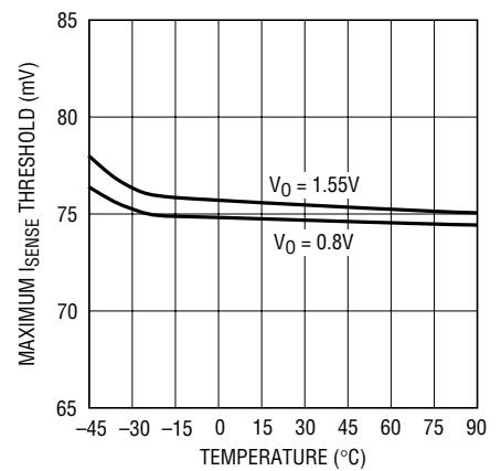
Maximum I_{SENSE} Threshold vs Temperature
