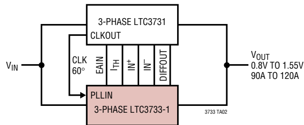
Block Diagram—6-Phase LTC3731/LTC3733-1 Supply
