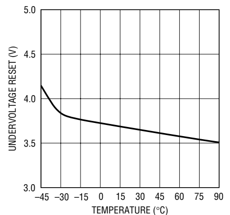
Undervoltage Reset Voltage vs Temperature
