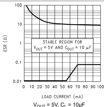
Figure 7-4. 5V, 10 \mu F ESR Curves (Legacy Chip)
