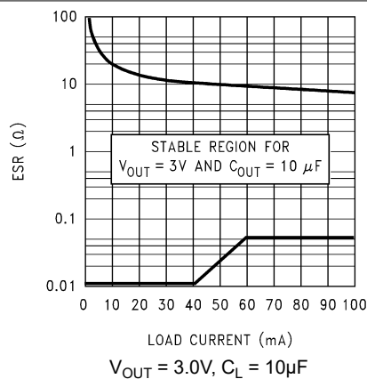
Figure 7-6. 3.0V, 10 \mu F ESR Curves (Legacy Chip)
