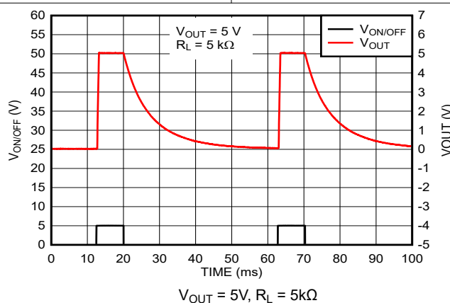
Figure 7-11. Turn-Off Waveform (New Chip)
