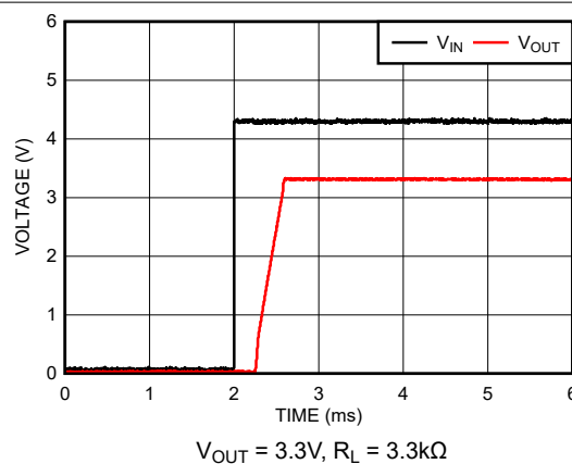
Figure 7-10. Turn-On Waveform (New Chip)
