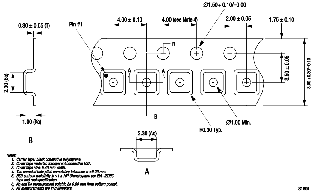
Figure 10. CLA4603-085LF Tape and Reel Dimensions
