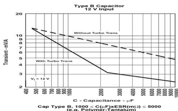
Type B TurboTrans C_o Values & Required R_{TT} Selection Table
