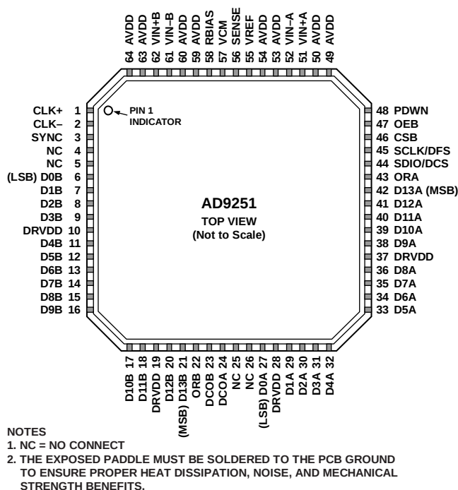
Figure 5. Pin Configuration
