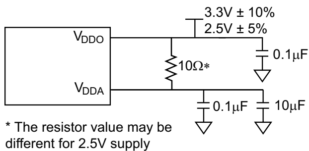
Figure 2. Power Supply Filter
