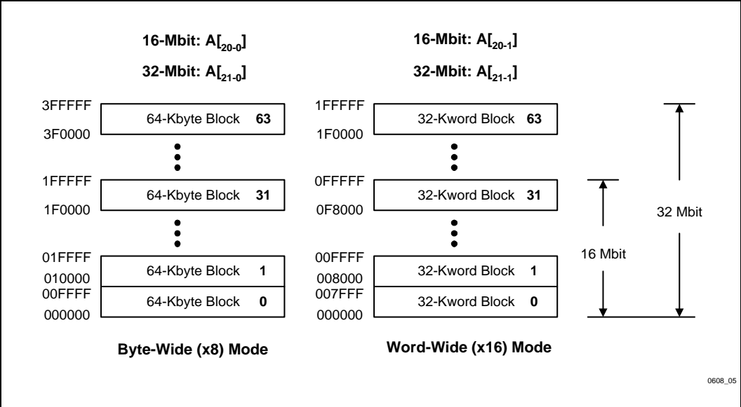
Figure 4. Memory Map
