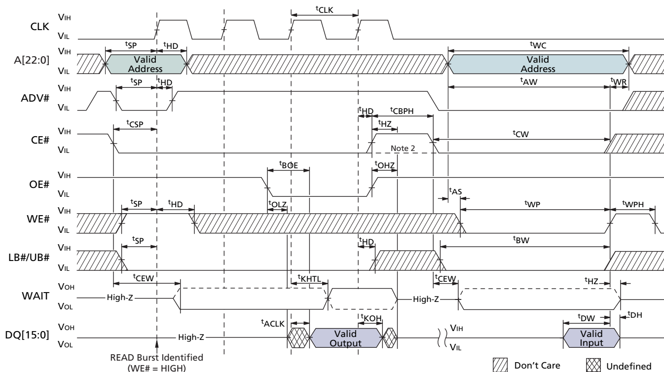
Figure 52: Burst READ Followed by Asynchronous WRITE (WE#-Controlled)
