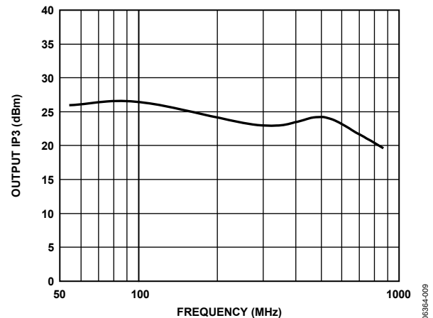
Figure 10. Output IP3 vs. Frequency
