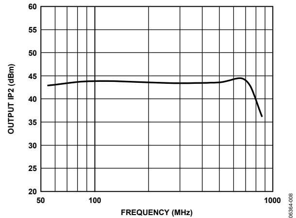
Figure 9. Output IP2 vs. Frequency
