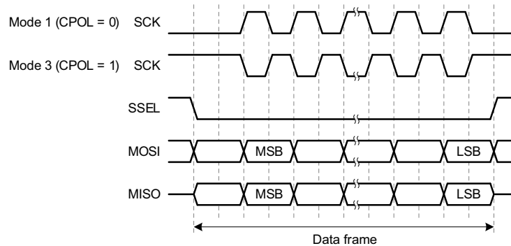
Fig 35. Basic SPI operating modes
