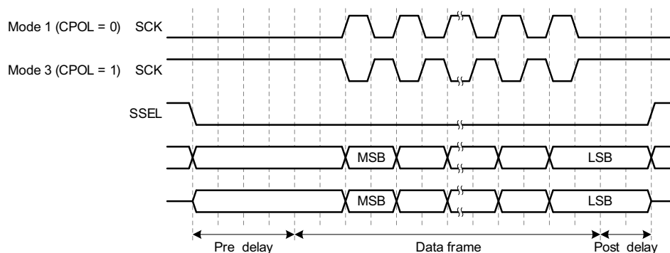
Fig 36. Pre_delay and Post_delay timing
