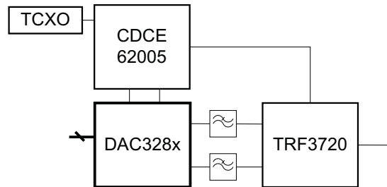
Figure 1. EVM Block Diagram
