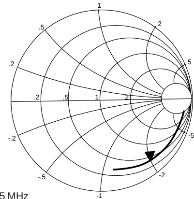
RF INPUT MATCH ( S_{11} )
