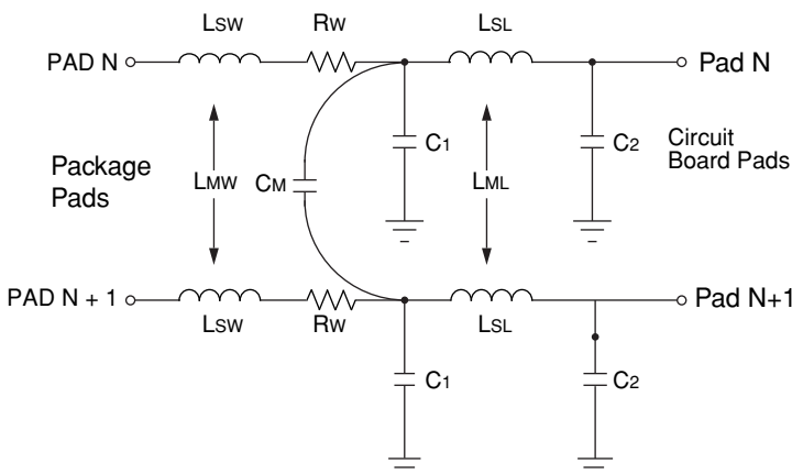
Figure 102. Package Parasitics
