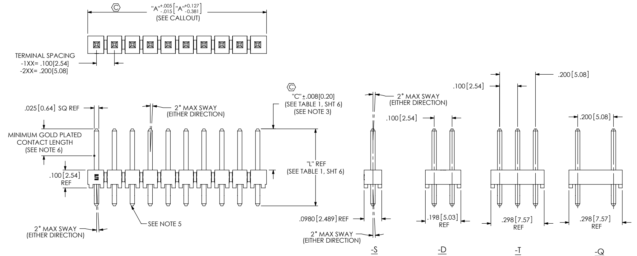
FIG 1 HTSW-110-07-XXX-D SHOWN
