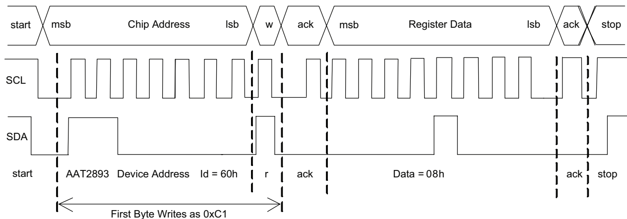
Figure 6: AAT2893 I²C Read Timing Diagram.
