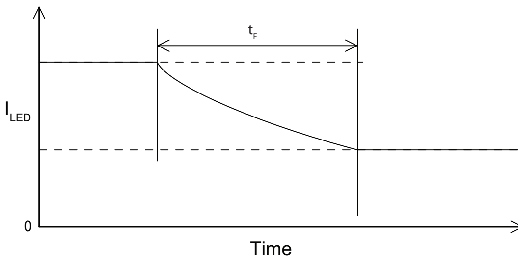
Figure 26: CABC Timing.
