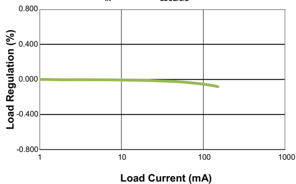
LDOB/C/D Output Voltage Load Regulation (V IN = 3.6V, V LDOB/C/D = 3.3V)
