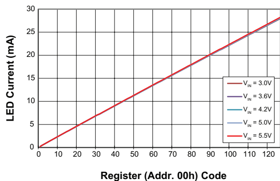
LED Current vs Register (Addr. 00h) Code (4.7 \mu H , 10 WLEDs)
