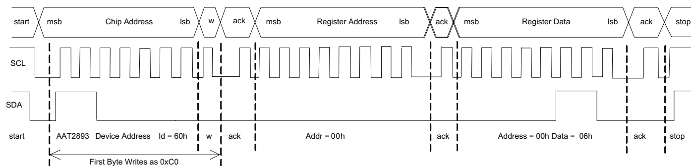
Figure 5: AAT2893 I²C Write Timing Diagram.
