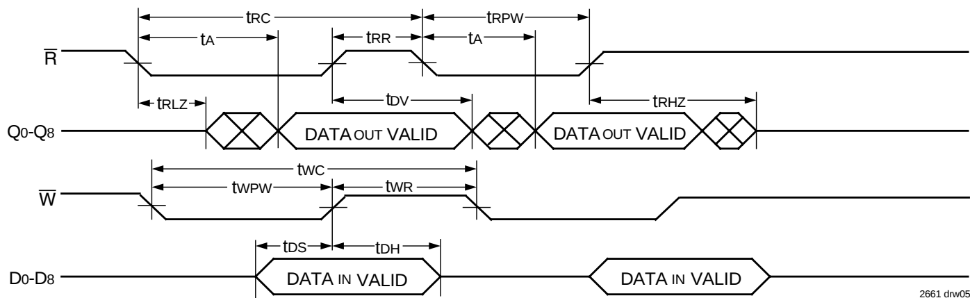
Figure 3. Asynchronous Write and Read Operation
