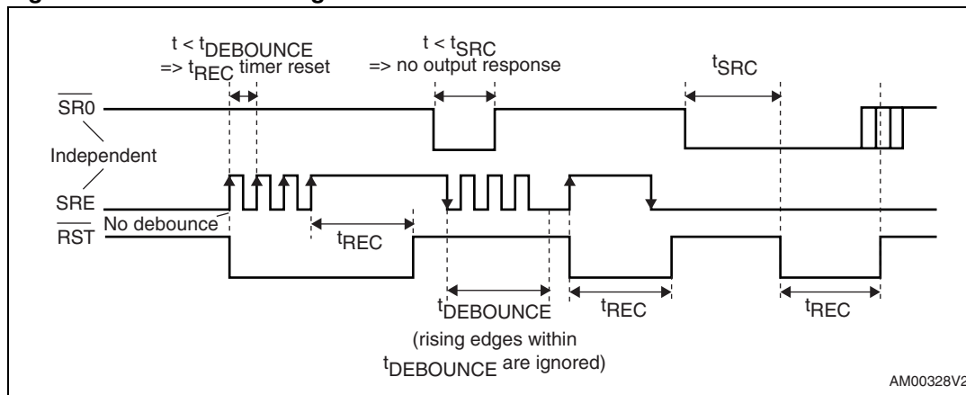
Figure 8. STM6504 timing
