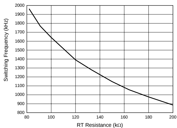
Figure 11. Switching Frequency vs. RT Resistance High Frequency Range
