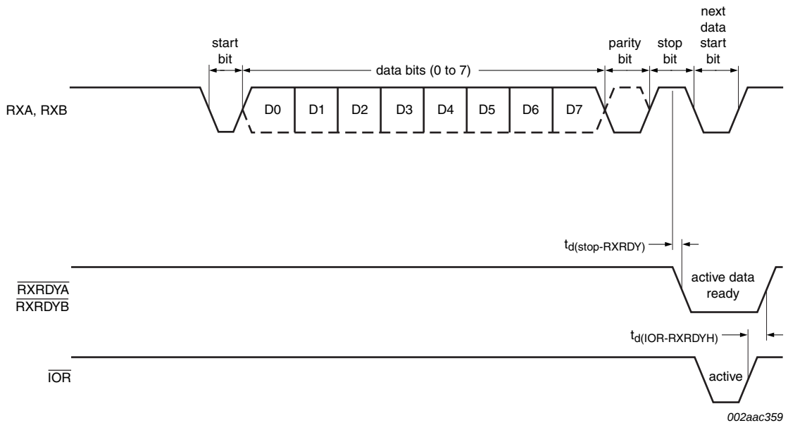
Fig 15. Receive ready timing in non-FIFO mode
