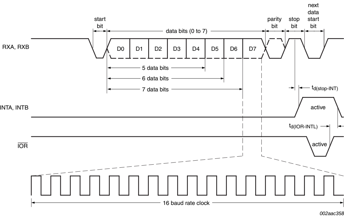
Fig 14. Receive timing
