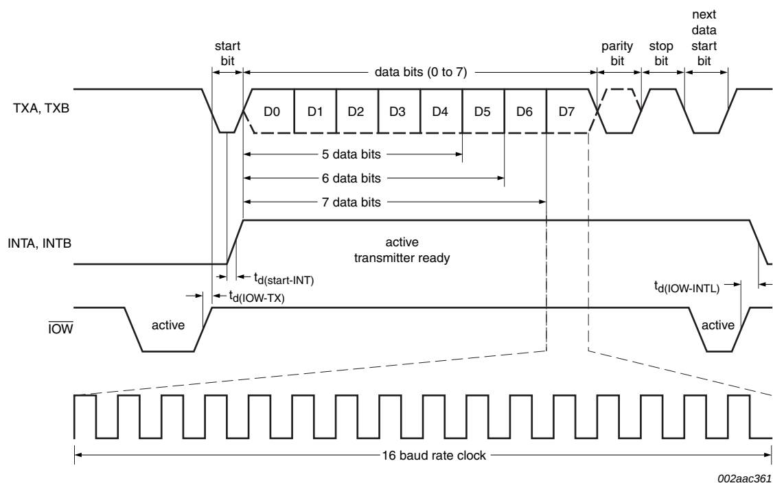
Fig 17. Transmit timing
