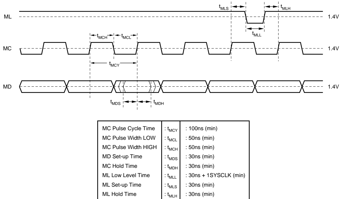
FIGURE 6. Program Register Input Timing.
