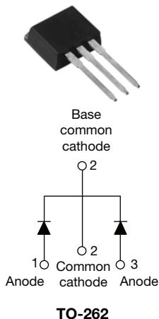
VS-40CTQ045-1PbF
